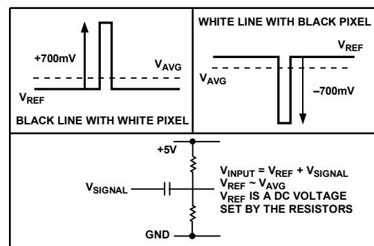
Figure 99. Pathological Case for Input Dynamic Range
